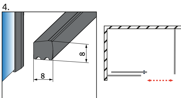
Wariant LEWY Variant L
